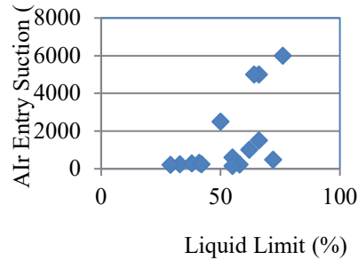
Fig 7 The liquid limit (L.L %) versus Air Entry Value (AEV)
