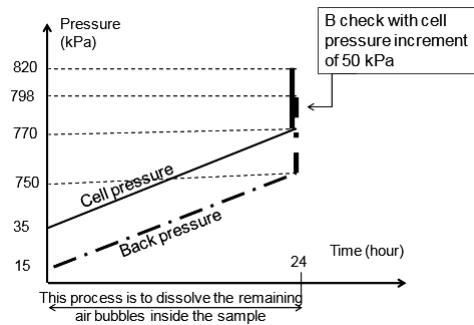
Figure 6. Ramp process to saturated the sample completely and B check
